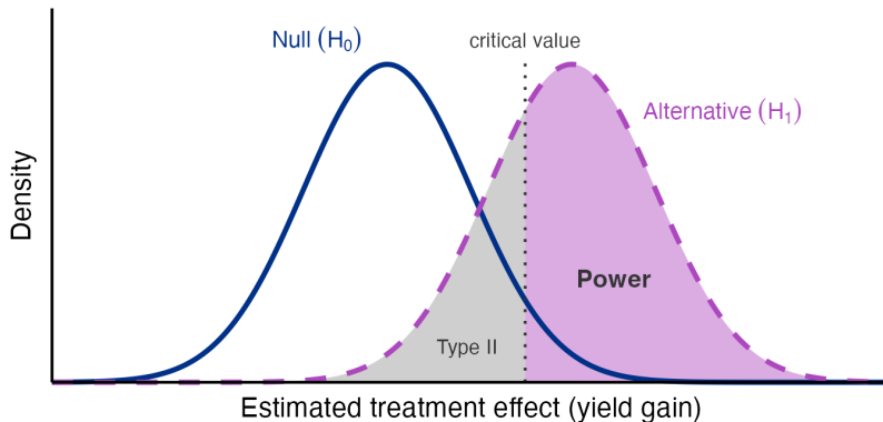
Figure 3: Power is the share of the alternative distribution that falls beyond the critical value. We can increase power by increasing the sample size.
