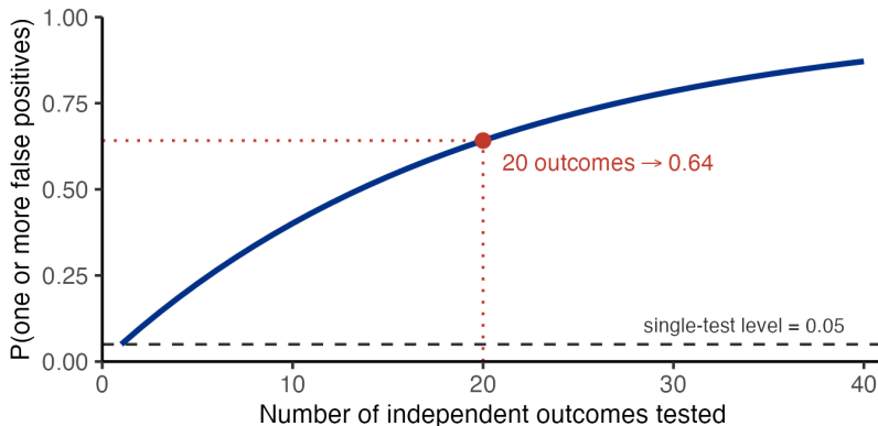
Figure 2: The chance of at least one false positive climbs quickly as we test more outcomes.
